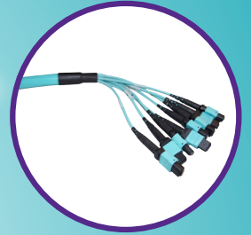
40G MTP® Trunk Cable PN: T96-PF3P2-PF32-4PMU-xxxM
